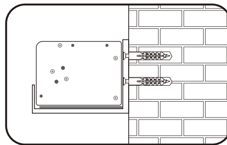
Schematic diagram of wall bracket accessories
